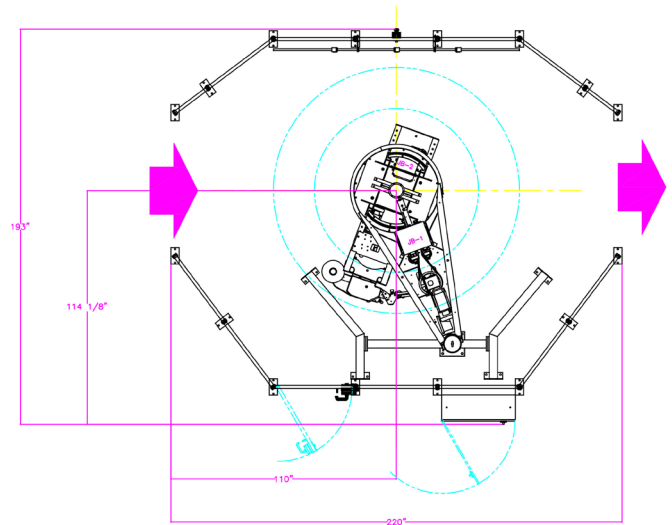
Reverse Flow: Shown with optional infeed, wrap zone, and exit conveyors
