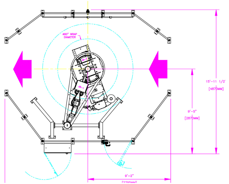
Standard Flow: Shown with optional infeed, wrap zone, and exit conveyors
